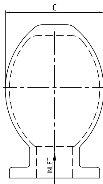
SECTION 'YY'
